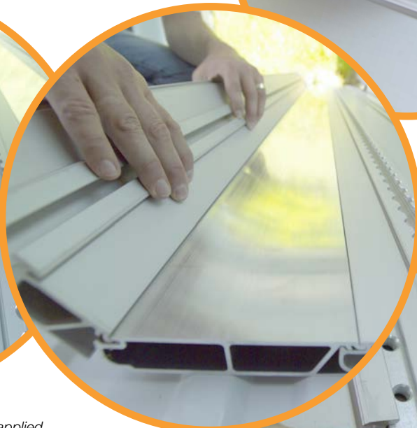
Rubber seal prevents dirt in the rails. Part no. 20000
